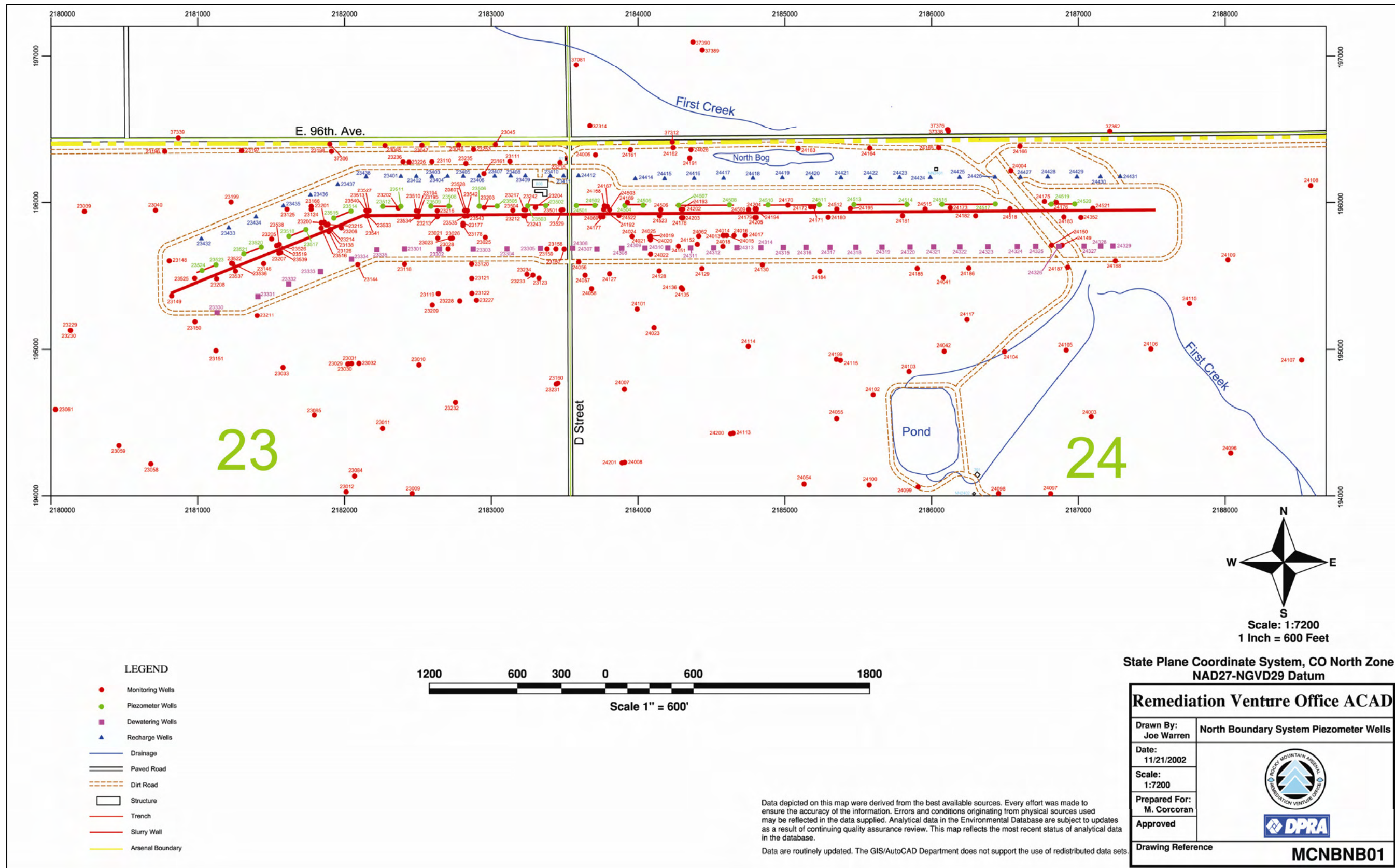
Figure 2. System configuration, NBCTS, November 2002
